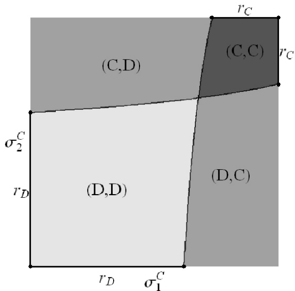
Figure 3: Basins of (potential) attraction for equilibria in the PD. \alpha = 2 .
