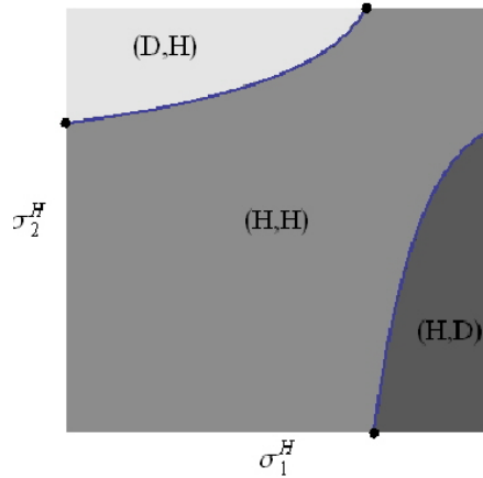
Figure 2: Best responses for an Hawk-Dove game with reciprocity.
