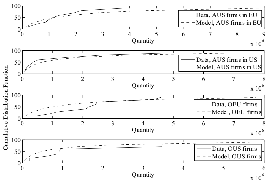
Figure 6: Quantity distributions
